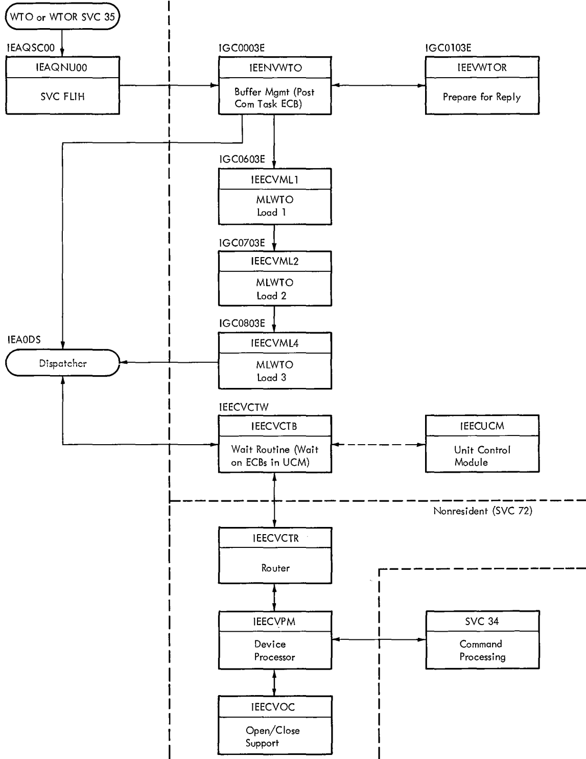
Figure 7-2. Console Support: Output
