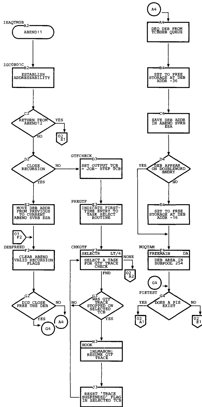
Chart LT. ABEND11 (Page 1 of 4)
