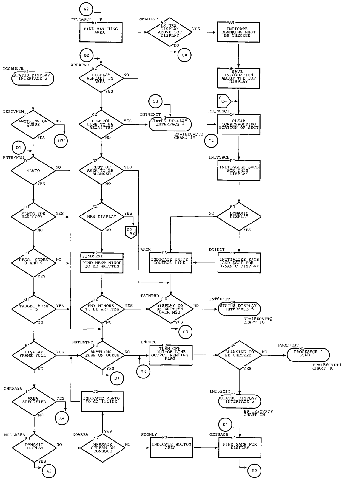
Chart IK. Status Display Interface 2 Routine (Page 1 of 2)
