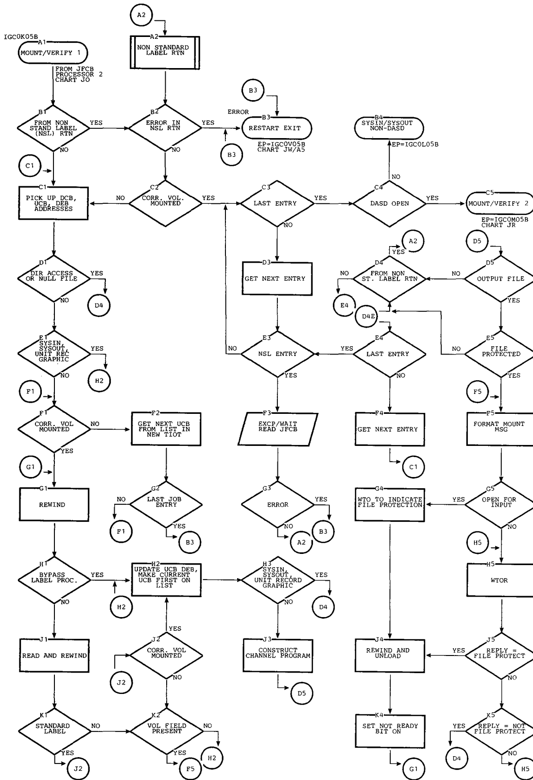
Chart JQ. Restart Mount Verify 1 Routine (Non-Direct Access)
