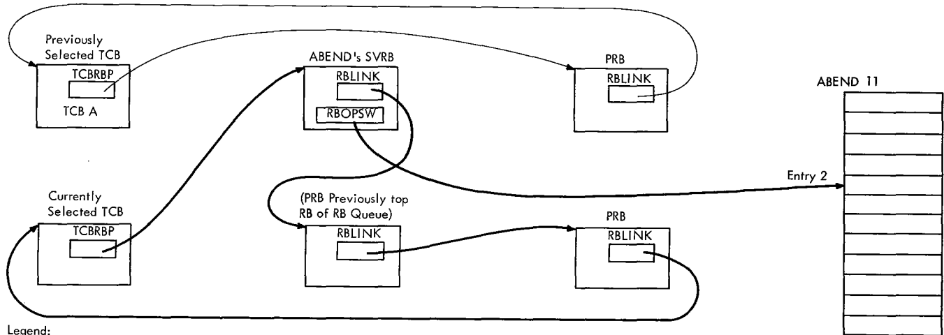
Figure 10-9. Preparation for the Dispatching of ABEND11 for the Selected Task
