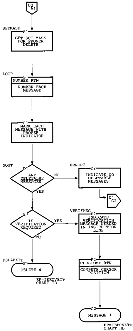
Chart IA. DIDOCS Delete 1 Routine (Page 2 of 2)
