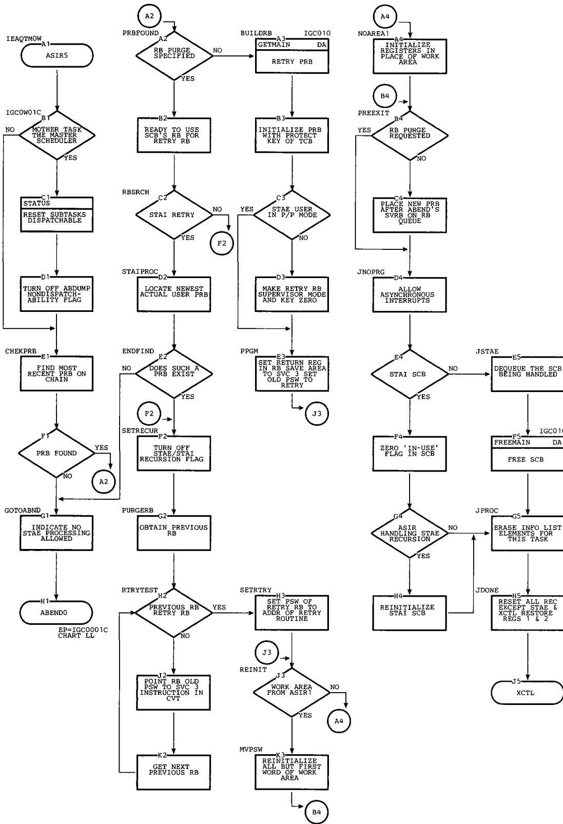
Chart BV. ABEND/STAE Interface 5 Routine (ASIR5)
