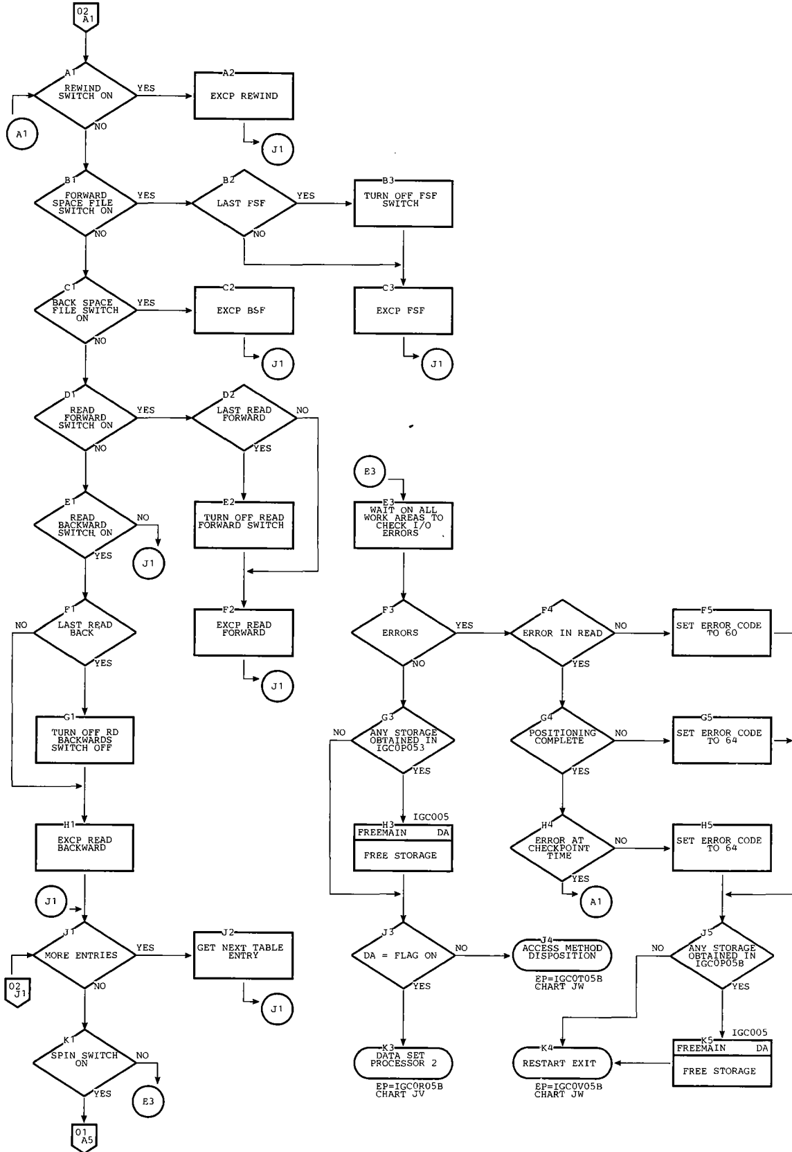
Chart JU. Restart Data Set Processor 1A -- Non-Direct Access (Page 2 of 2)
