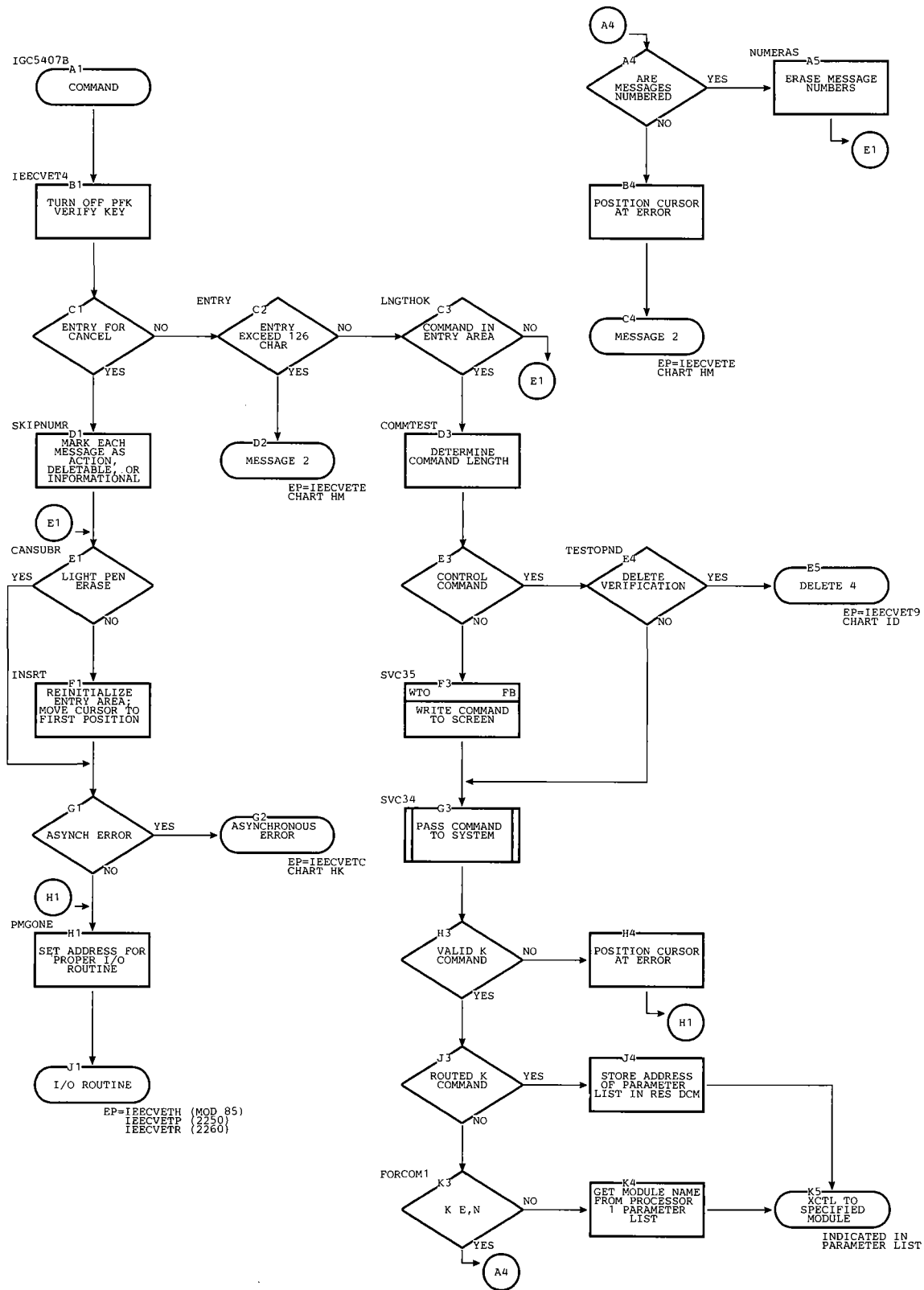
Chart HS. DIDOCS Command Routine
