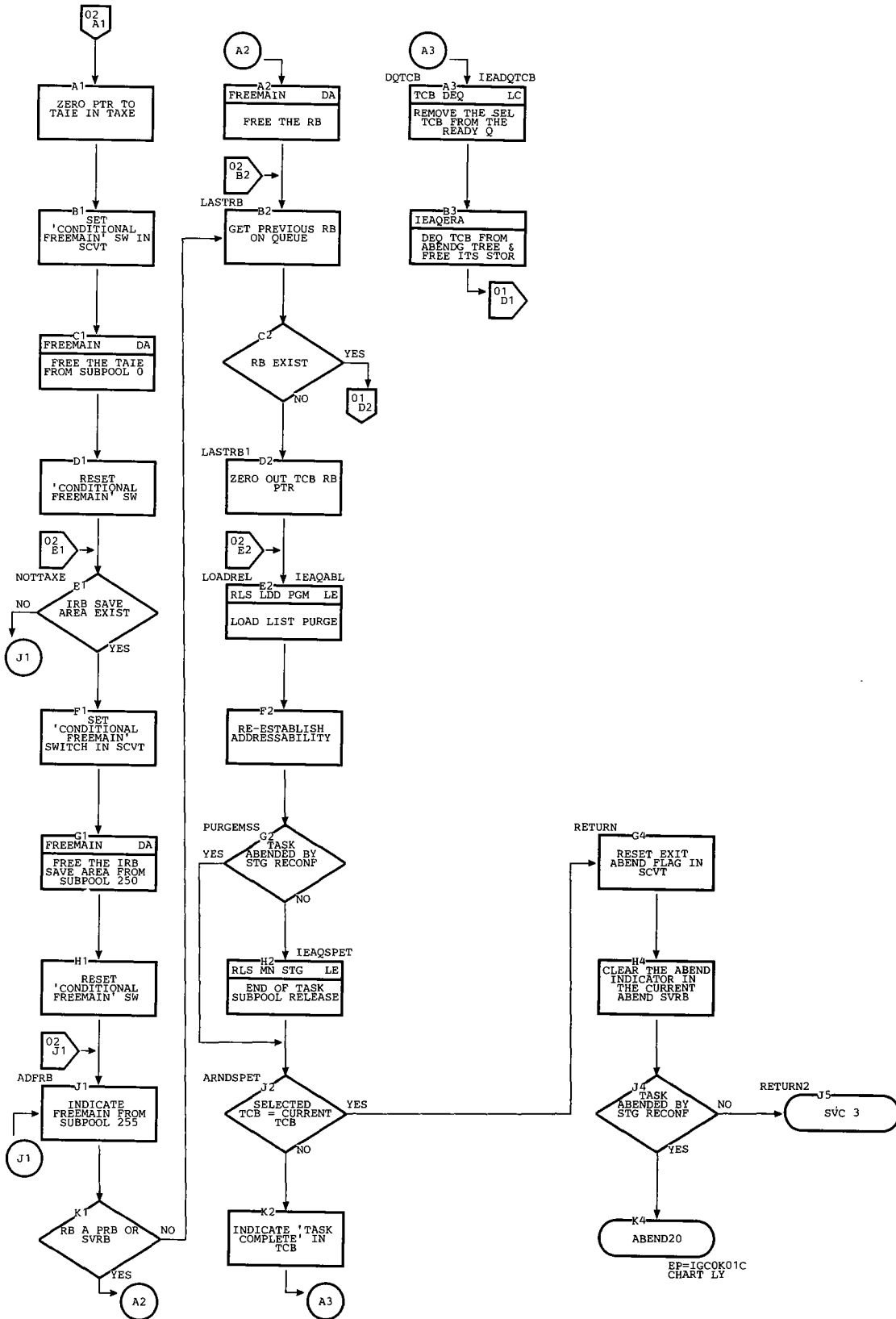
Chart LX. ABEND16 (Page 2 of 2)
